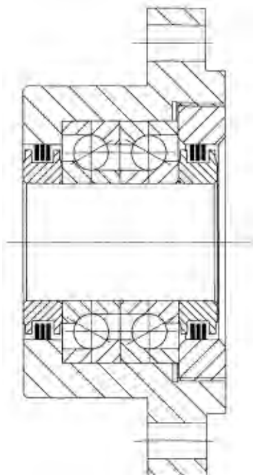
MOD. DUPLEX
